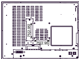
PS3711A-T42-24V Rear
