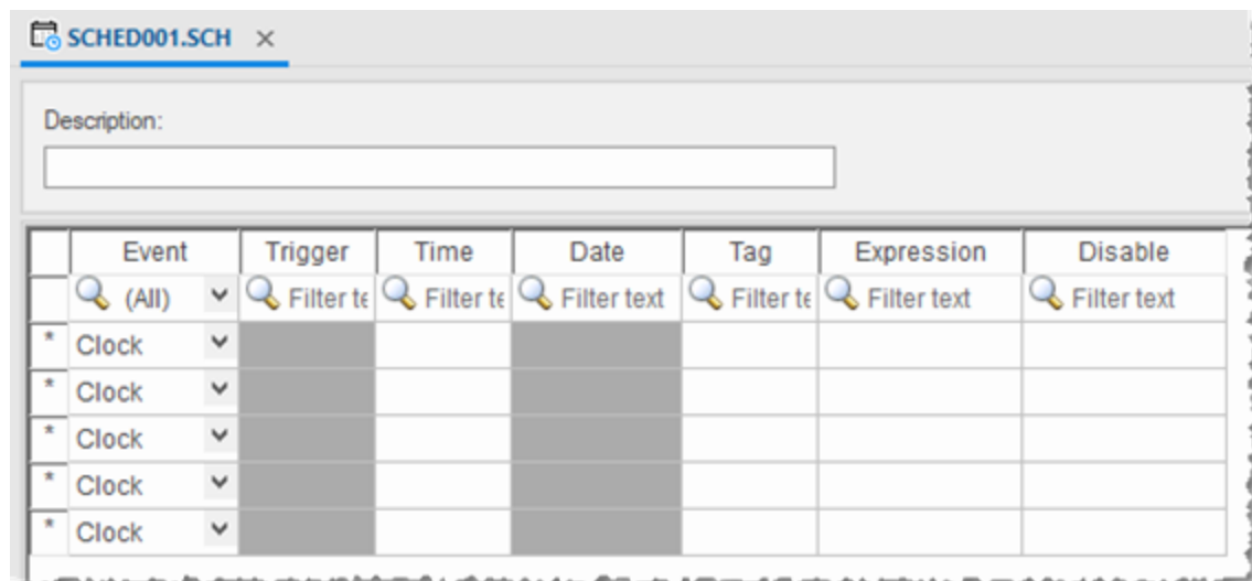
Scheduler worksheet
