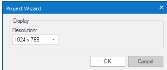
Project Wizard
