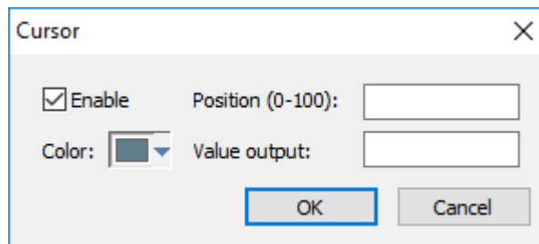
Cursor Dialog
