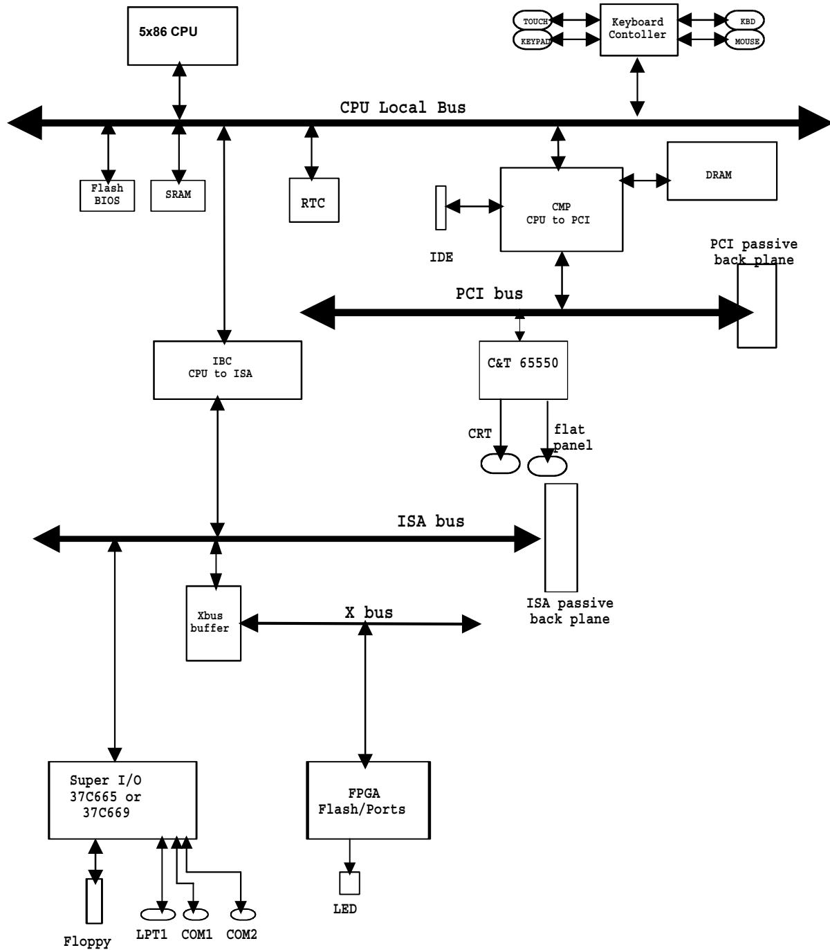
Figure Chapter 1 -1. Functional block diagram-AHIP4+
