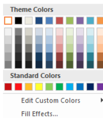
Color picker
