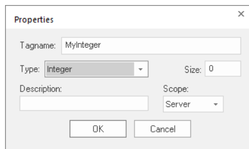
Properties dialog
