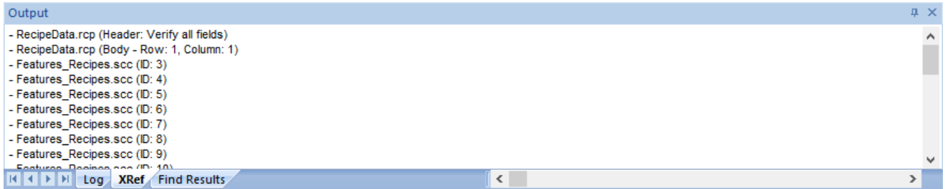
XRef Results
