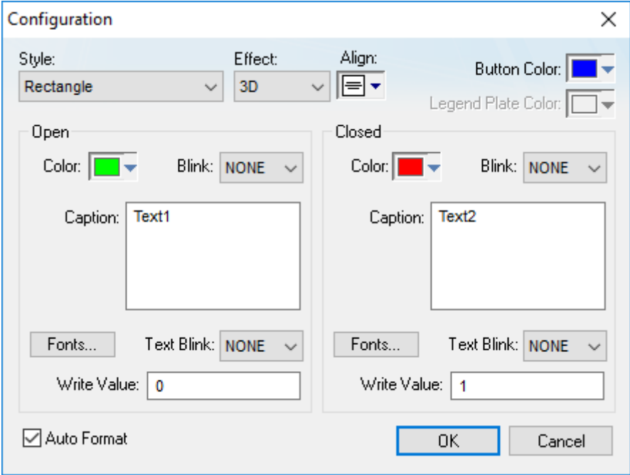
Configuration dialog
