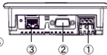
GP-3200T/A Bottom
